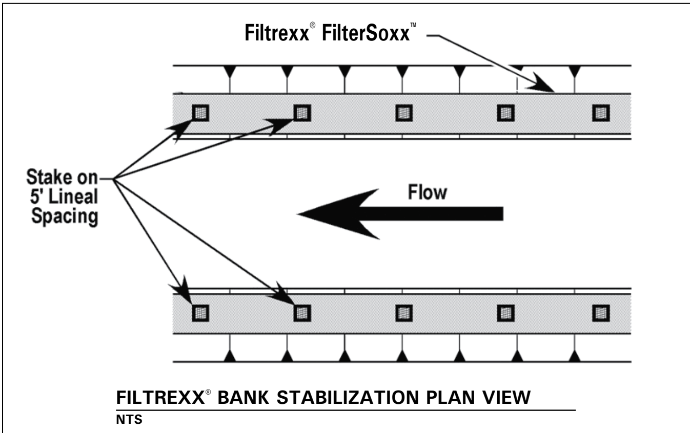
Figure 5.3. Staking Details for Filtrexx® Bank Stabilization
