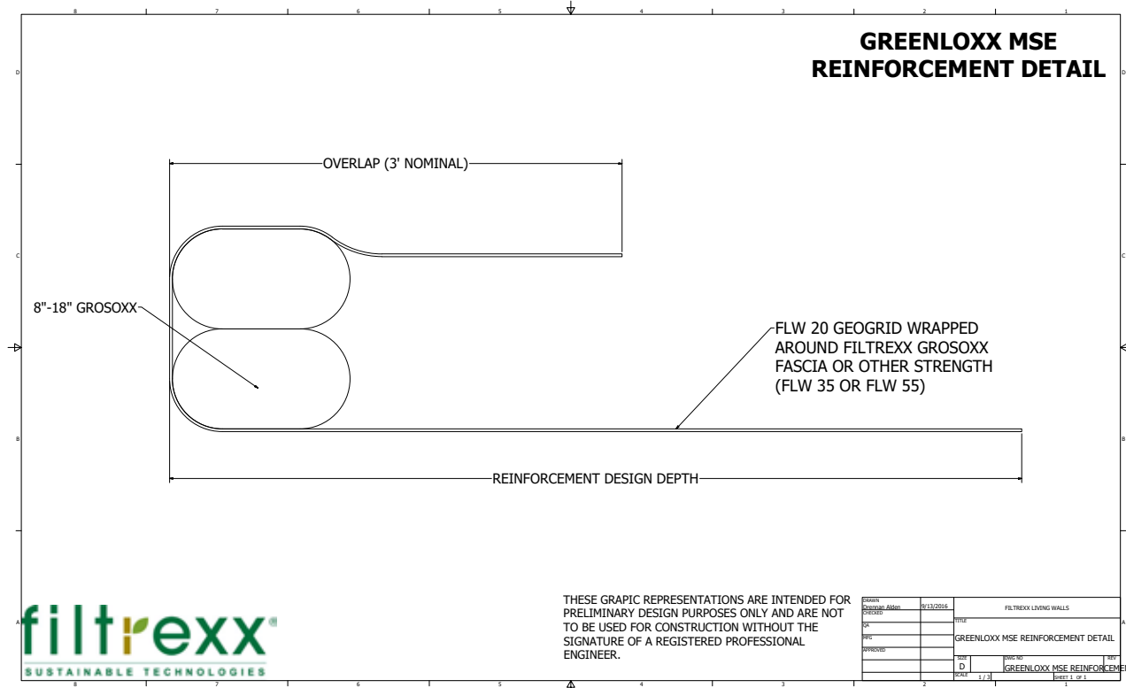
Figure 2.3. Filtrexx® GreenLoxx® MSE Reinforcement Detail
