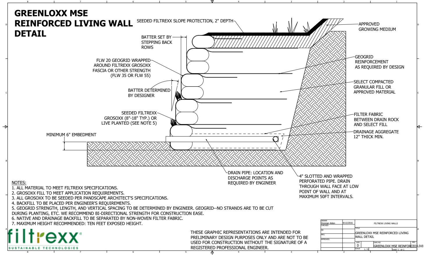
Figure 2.1. Engineering Design Drawing for Filtrexx GreenLoxx® MSE Retaining Living Wall
