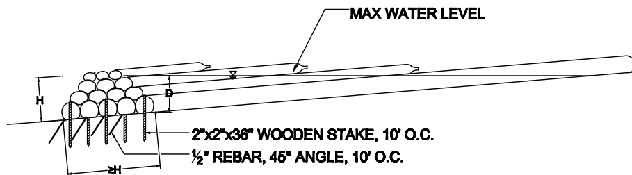
SECTION
