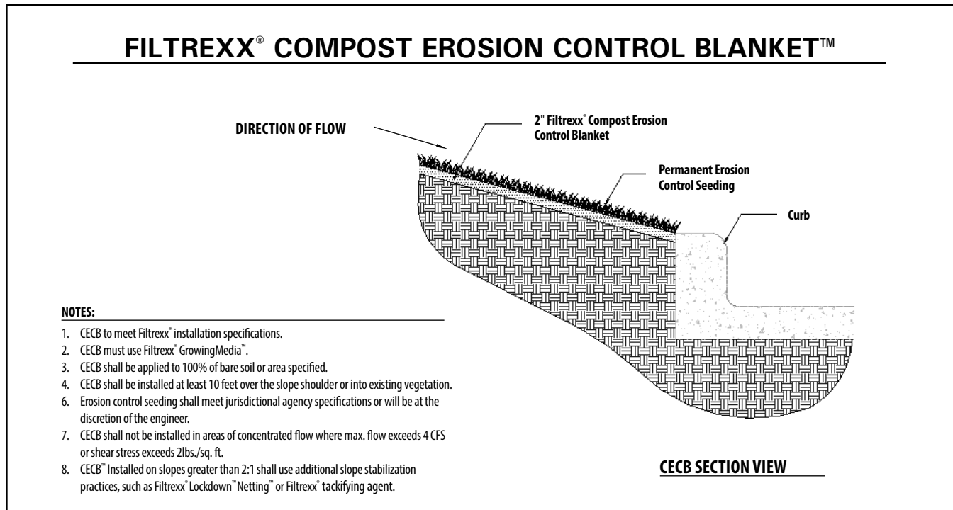
Figure 8.1. Engineering Design Details for Compost Erosion Control Blanket [CECB]
