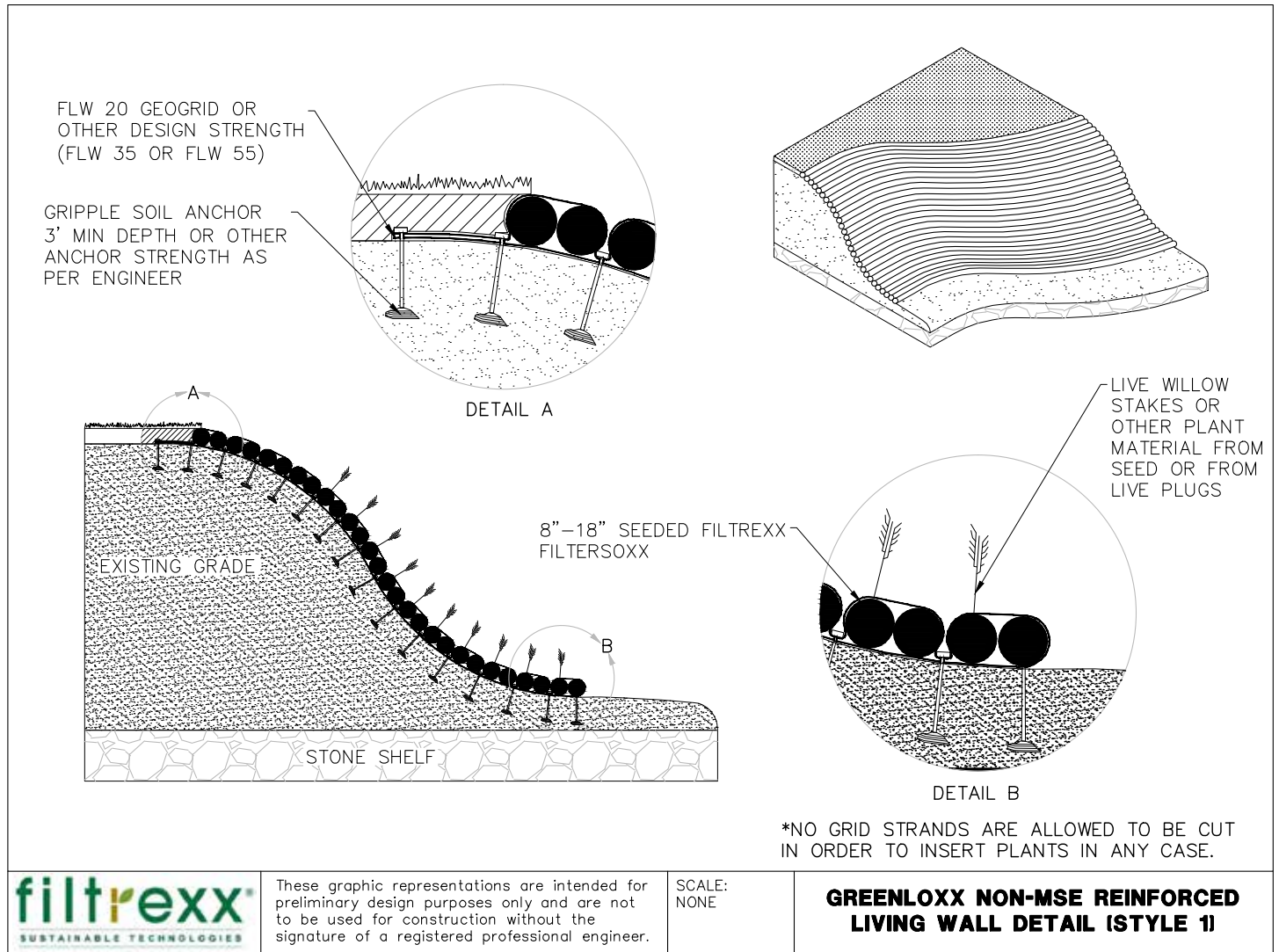
Figure 1.1. Engineering Design Drawing for Filtrexx GreenLoxx® Non-MSE Living Wall
