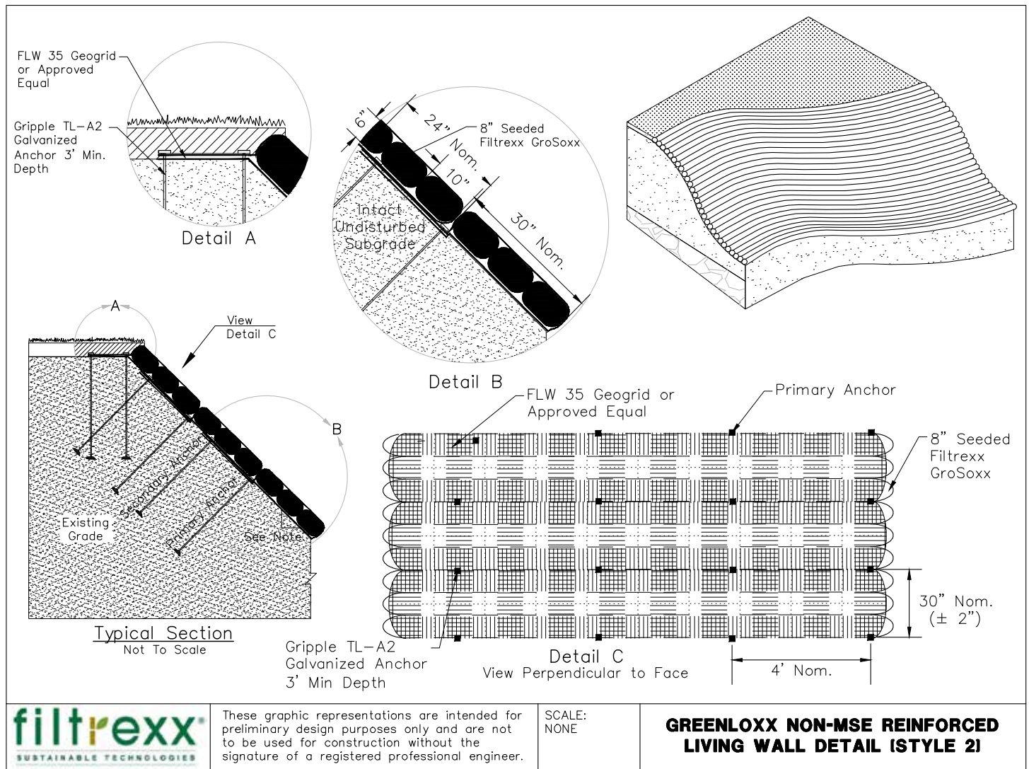
Figure 1.2. Engineering Design Drawings for Filtrexx GreenLoxx® Non-MSE Living Wall - Alternate Drawing
