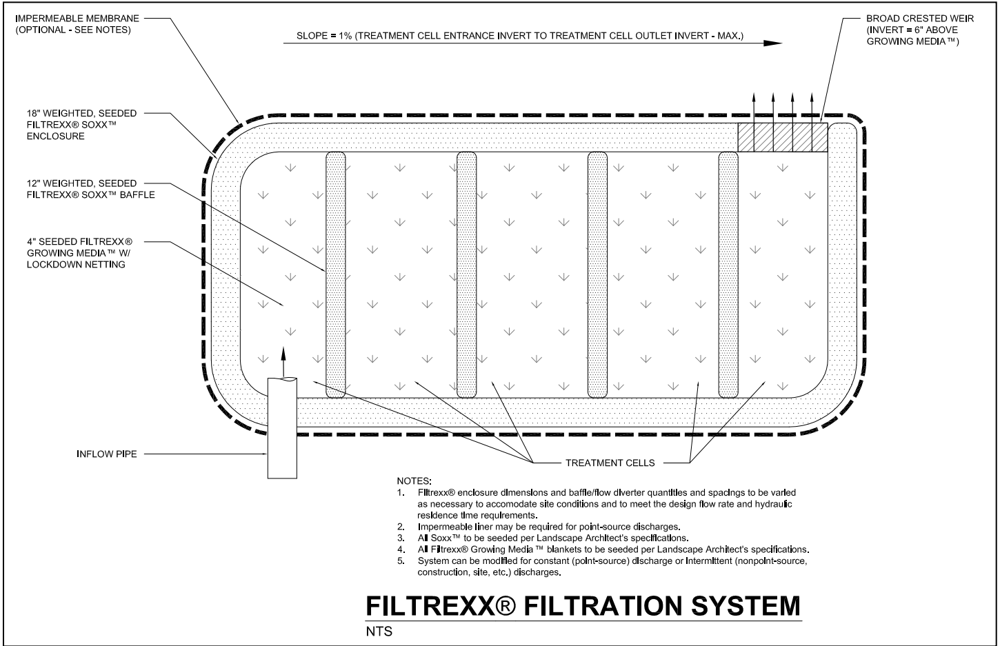
Figure 6.1. Engineering Design Drawings for Filtrexx® Filtration System - Option 1
